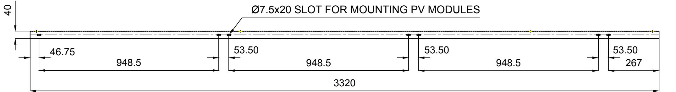
TOP VIEW
