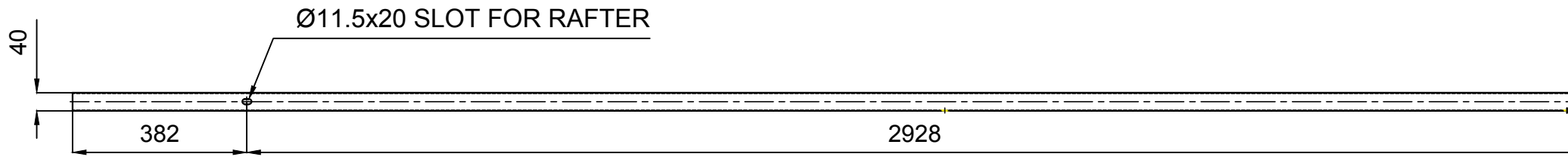
BOTTOM VIEW
