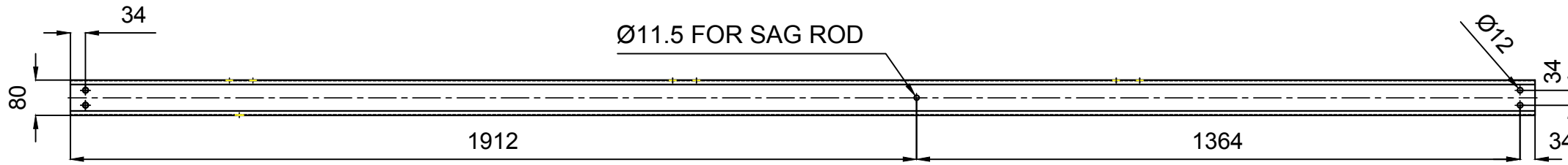
FRONT VIEW
