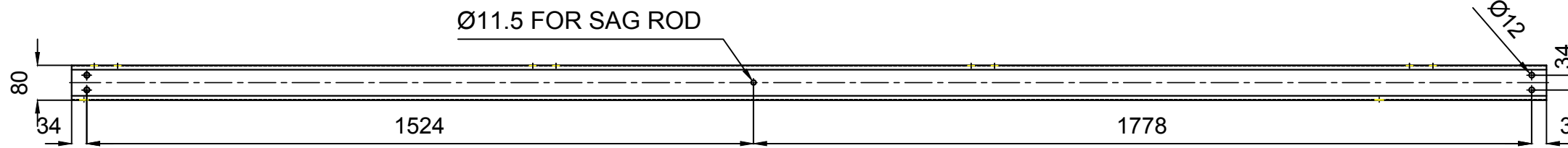
FRONT VIEW
